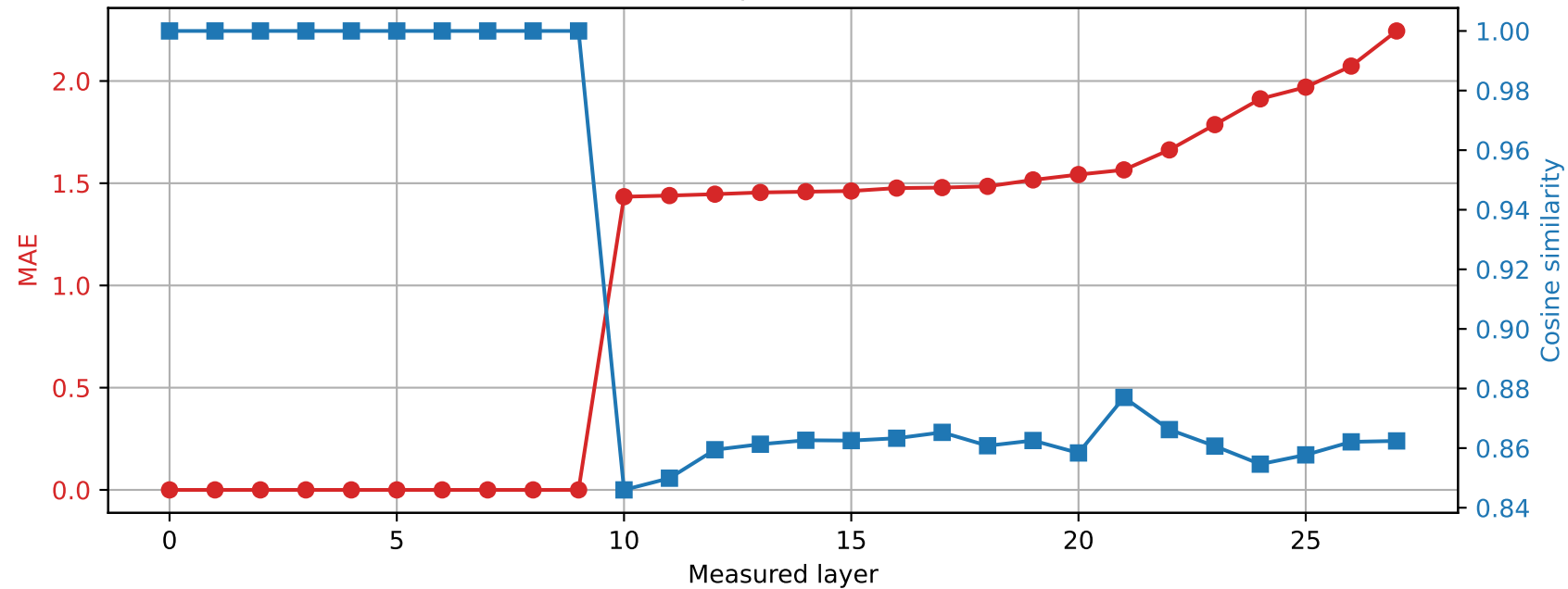
Qwen2.5-7B-Instruct | Prompt 0 Spared layer 9 | Hybrid vs quantized
