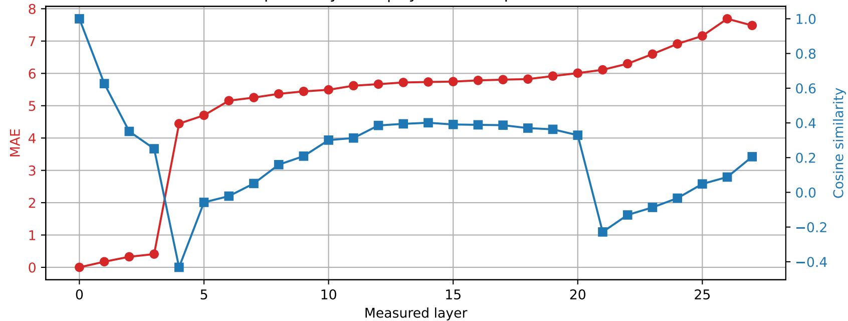
Qwen2.5-7B-Instruct | Prompt 0 Spared layer 10 | Hybrid vs unquantized
