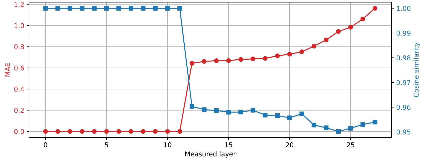
Qwen2.5-7B-Instruct | Prompt 0 Spared layer 11 | Hybrid vs quantized
