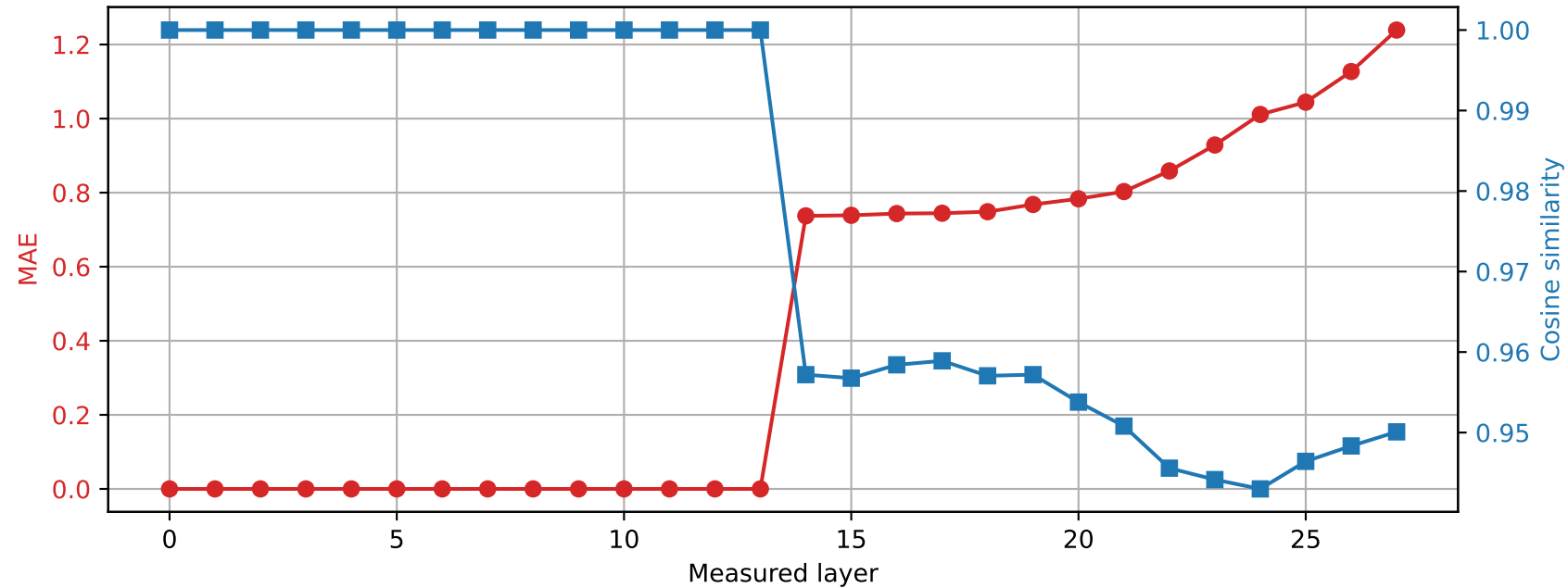
Qwen2.5-7B-Instruct | Prompt 0 Spared layer 13 | Hybrid vs quantized
