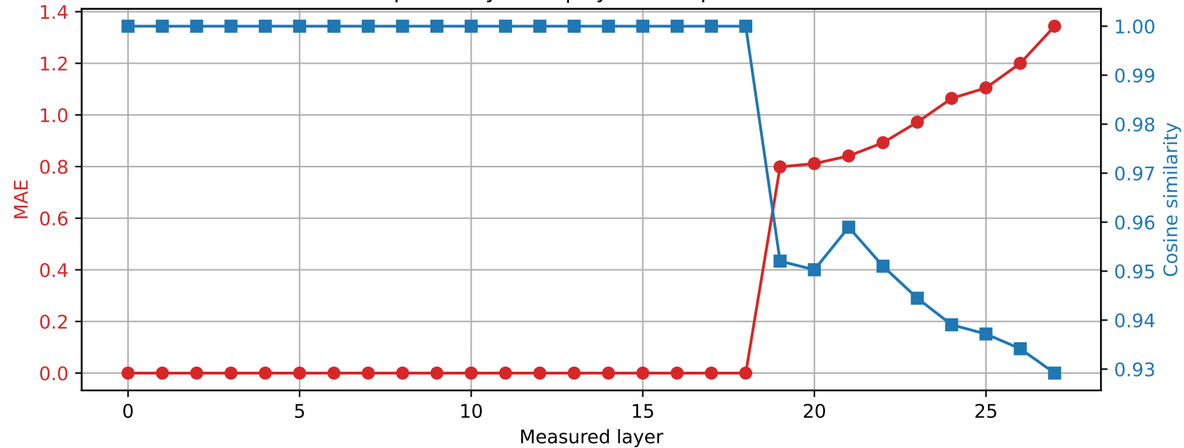
Qwen2.5-7B-Instruct | Prompt 0 Spared layer 18 | Hybrid vs quantized
