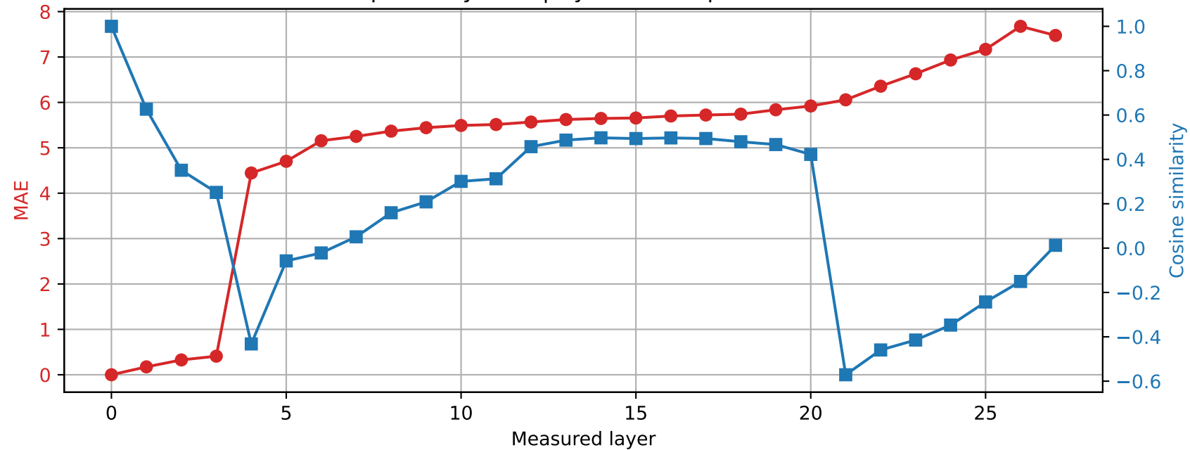
Qwen2.5-7B-Instruct | Prompt 0 Spared layer 21 | Hybrid vs unquantized
