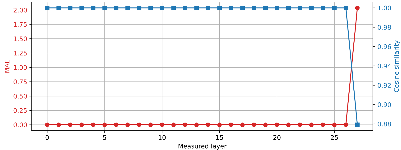
Qwen2.5-7B-Instruct | Prompt 0 Spared layer 26 | Hybrid vs quantized
