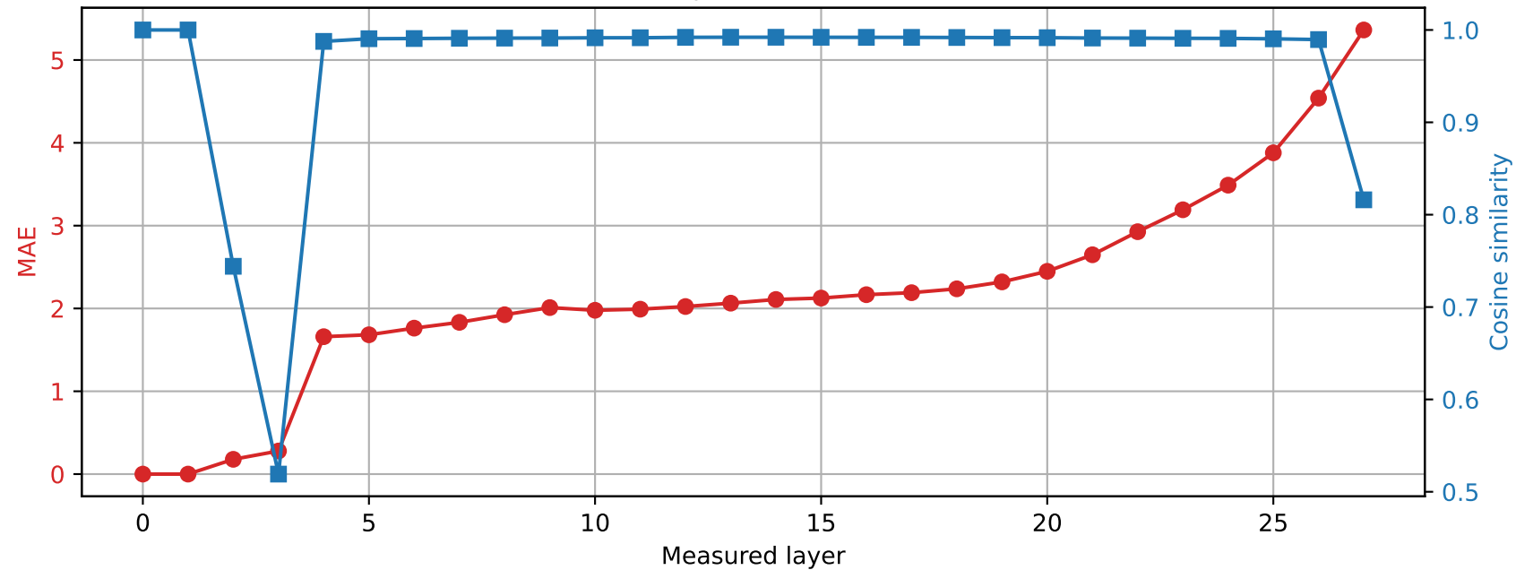
Qwen2.5-7B-Instruct | Prompt 1 Spared layer 0 | Hybrid vs unquantized
