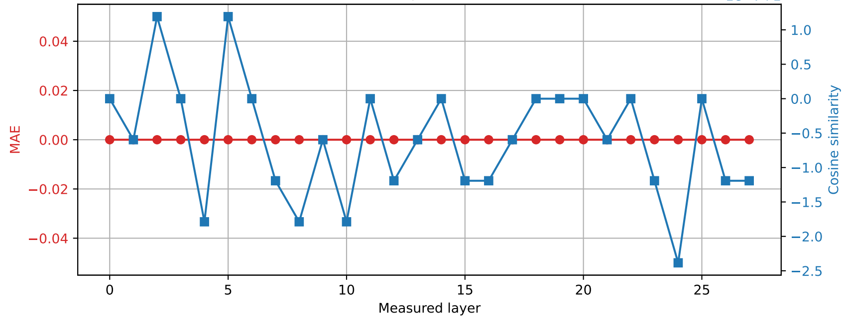
Qwen2.5-7B-Instruct | Prompt 1 Spared layer 27 | Hybrid vs quantized
