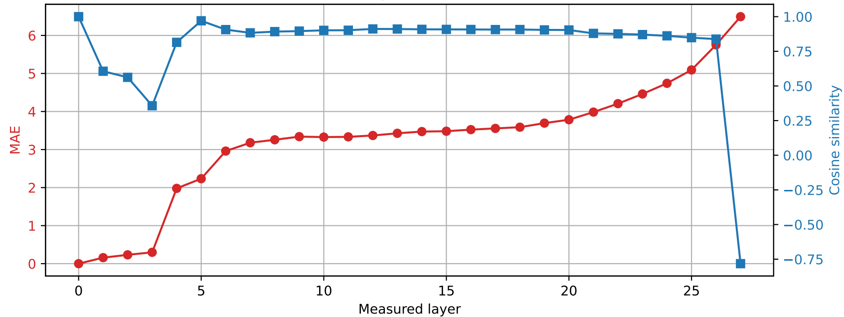
Qwen2.5-7B-Instruct | Prompt 1 Spared layer 27 | Hybrid vs unquantized
