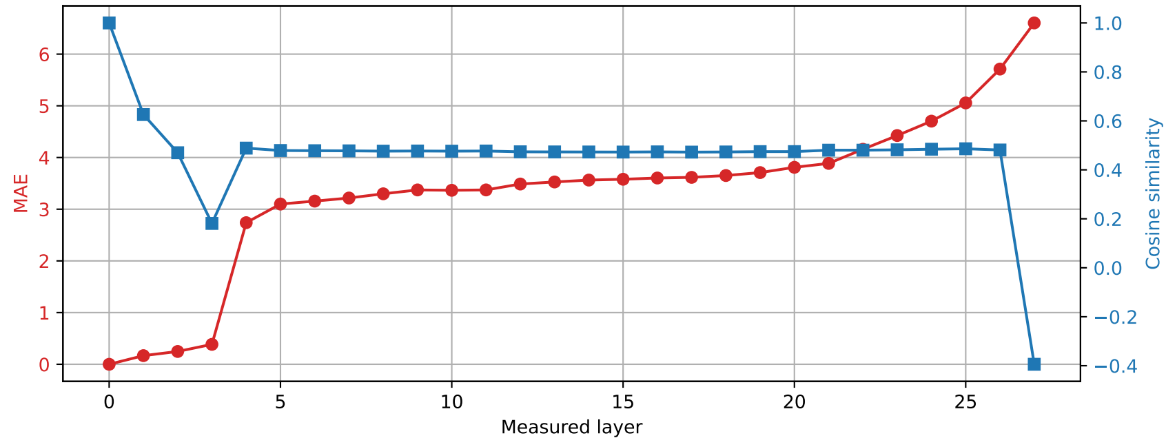
Qwen2.5-7B-Instruct | Prompt 2 Unquantized vs quantized int4
