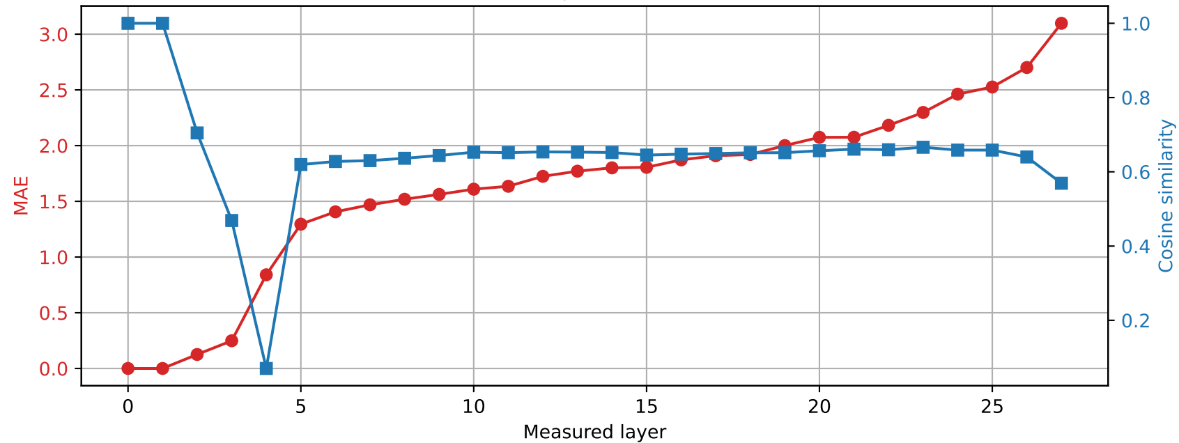
Qwen2.5-7B-Instruct | Prompt 2 Spared layer 1 | Hybrid vs quantized
