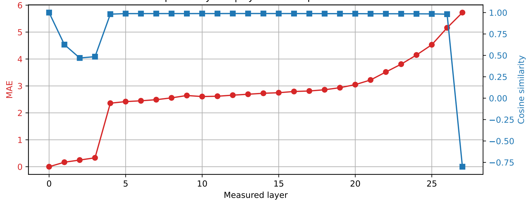
Qwen2.5-7B-Instruct | Prompt 2 Spared layer 2 | Hybrid vs unquantized
