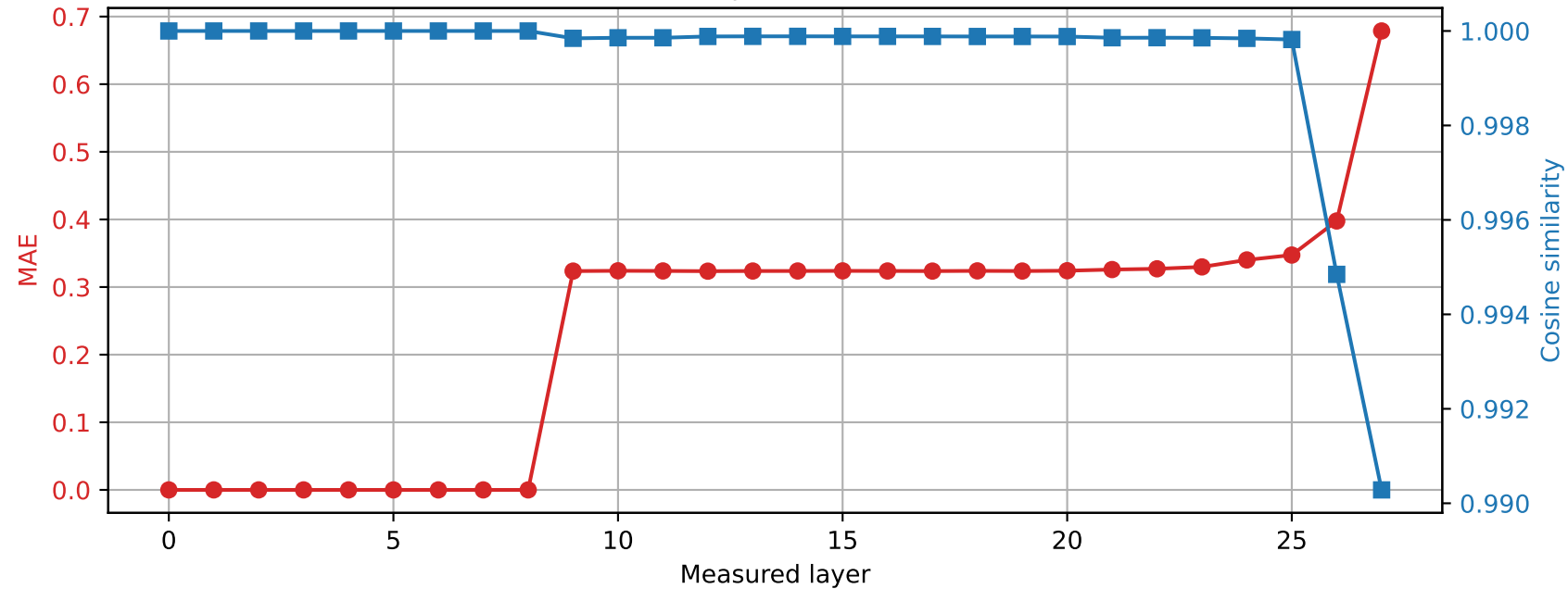
Qwen2.5-7B-Instruct | Prompt 2 Spared layer 8 | Hybrid vs quantized
