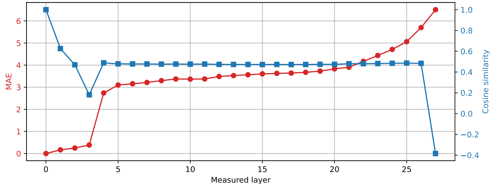
Qwen2.5-7B-Instruct | Prompt 2 Spared layer 14 | Hybrid vs unquantized
