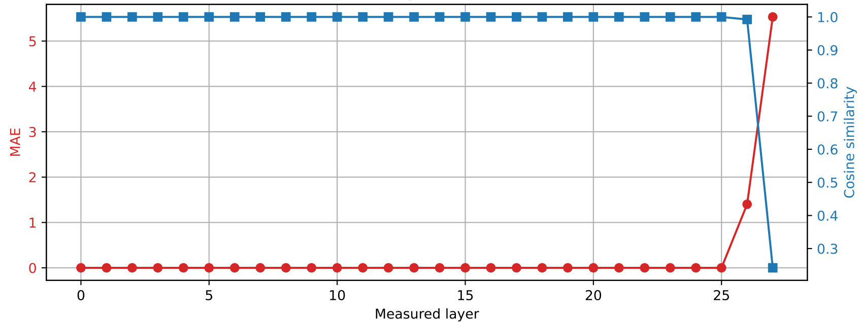
Qwen2.5-7B-Instruct | Prompt 2 Spared layer 25 | Hybrid vs quantized
