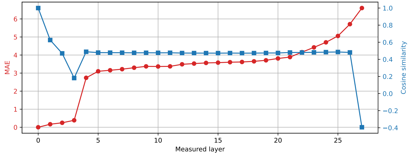
Qwen2.5-7B-Instruct | Prompt 2 Spared layer 27 | Hybrid vs unquantized
