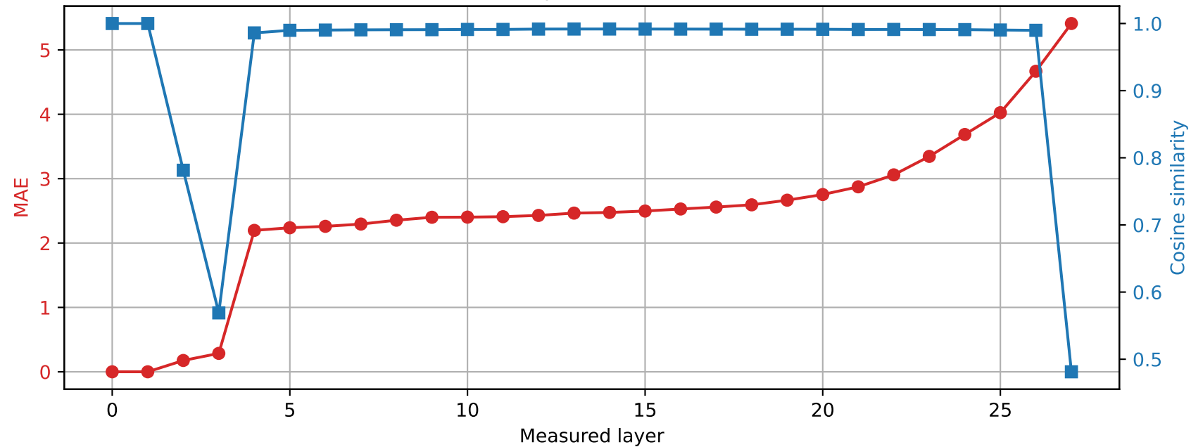
Qwen2.5-7B-Instruct | Prompt 3 Spared layer 0 | Hybrid vs unquantized
