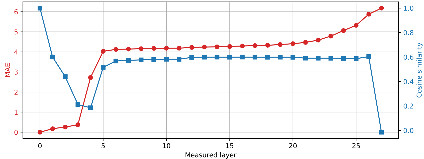
Qwen2.5-7B-Instruct | Prompt 3 Spared layer 4 | Hybrid vs unquantized
