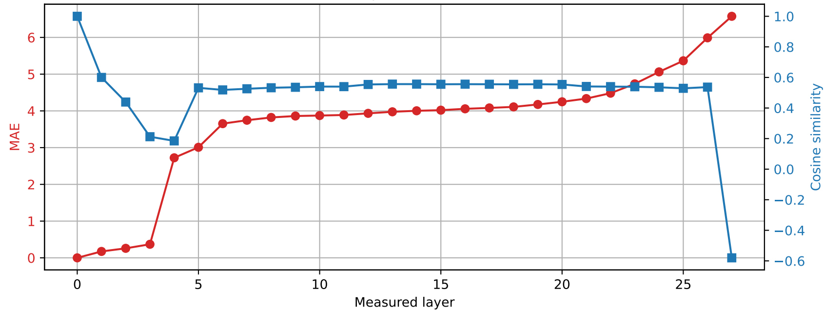
Qwen2.5-7B-Instruct | Prompt 3 Spared layer 7 | Hybrid vs unquantized
