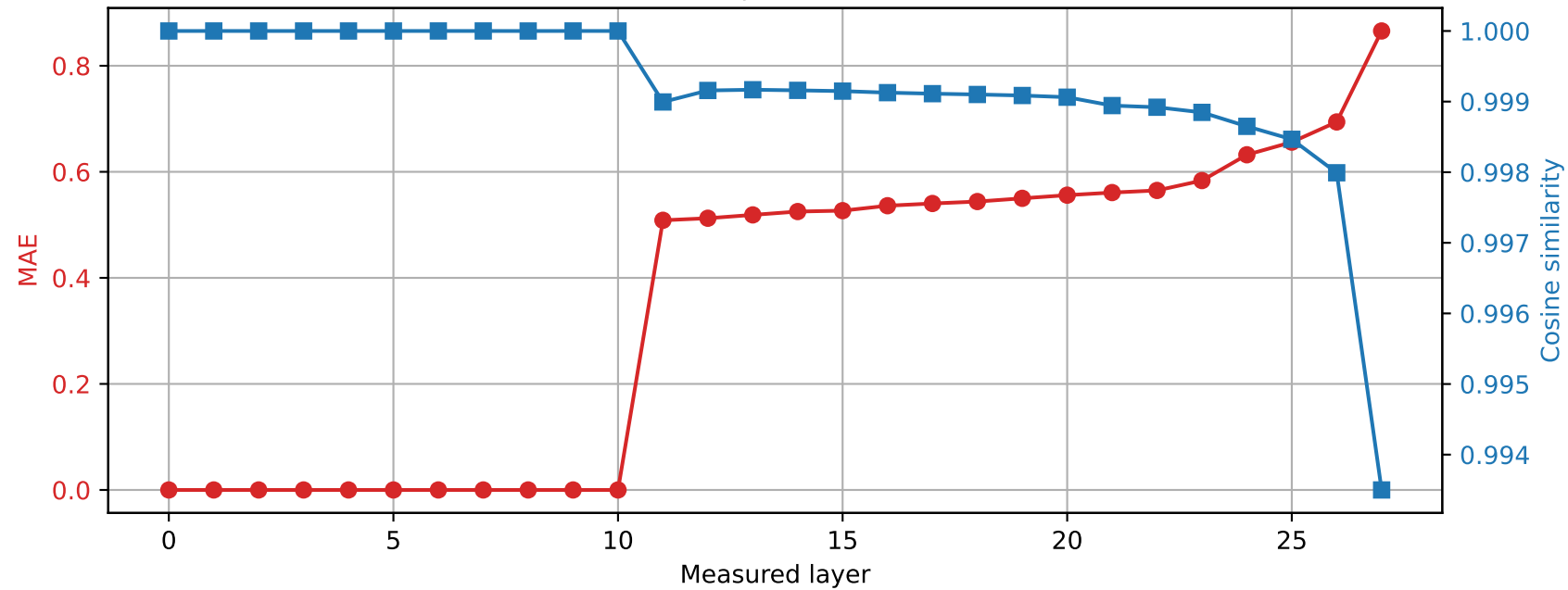
Qwen2.5-7B-Instruct | Prompt 3 Spared layer 10 | Hybrid vs quantized
