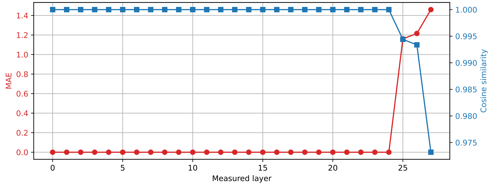
Qwen2.5-7B-Instruct | Prompt 3 Spared layer 24 | Hybrid vs quantized
