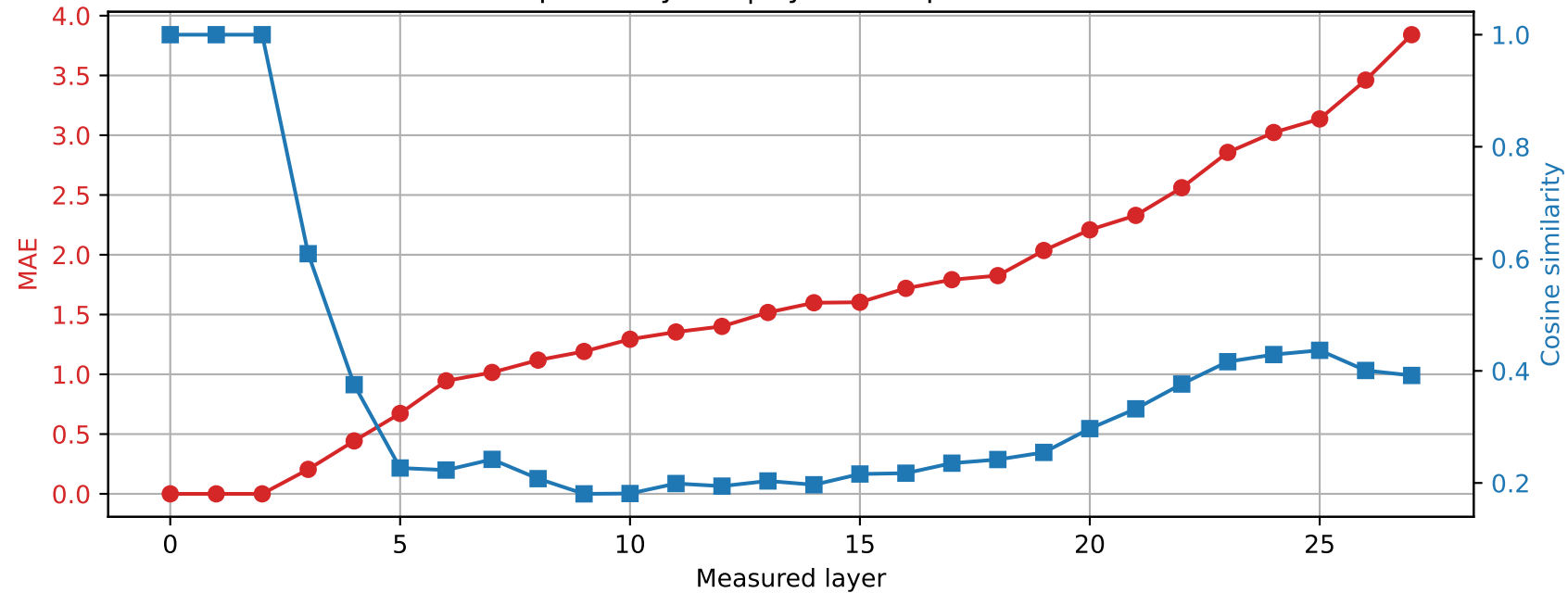
Qwen2.5-7B-Instruct | Prompt 4 Spared layer 2 | Hybrid vs quantized
