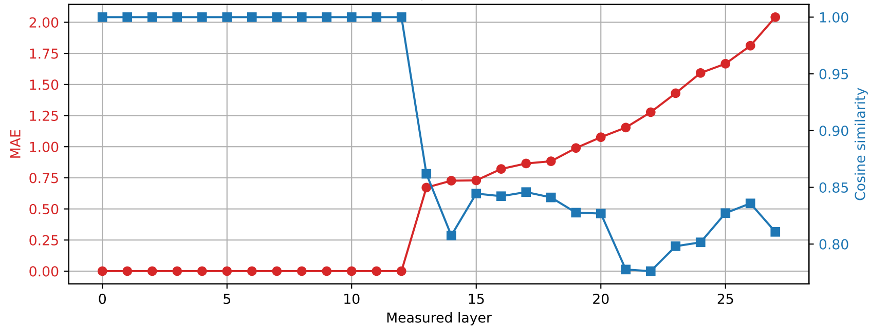
Qwen2.5-7B-Instruct | Prompt 4 Spared layer 12 | Hybrid vs quantized
