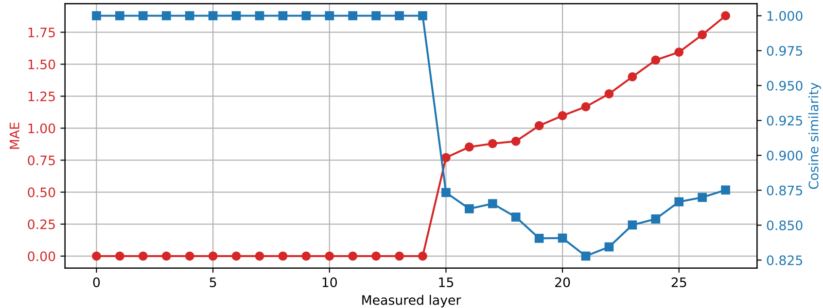
Qwen2.5-7B-Instruct | Prompt 4 Spared layer 14 | Hybrid vs quantized
