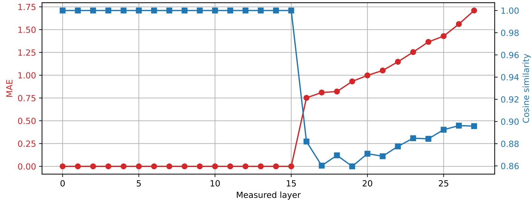
Qwen2.5-7B-Instruct | Prompt 4 Spared layer 15 | Hybrid vs quantized
