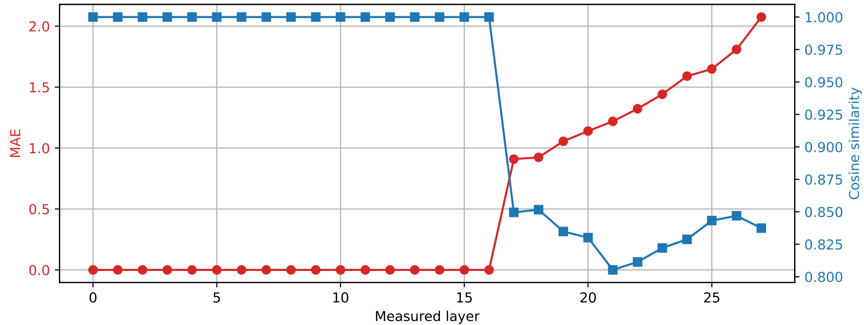
Qwen2.5-7B-Instruct | Prompt 4 Spared layer 16 | Hybrid vs quantized
