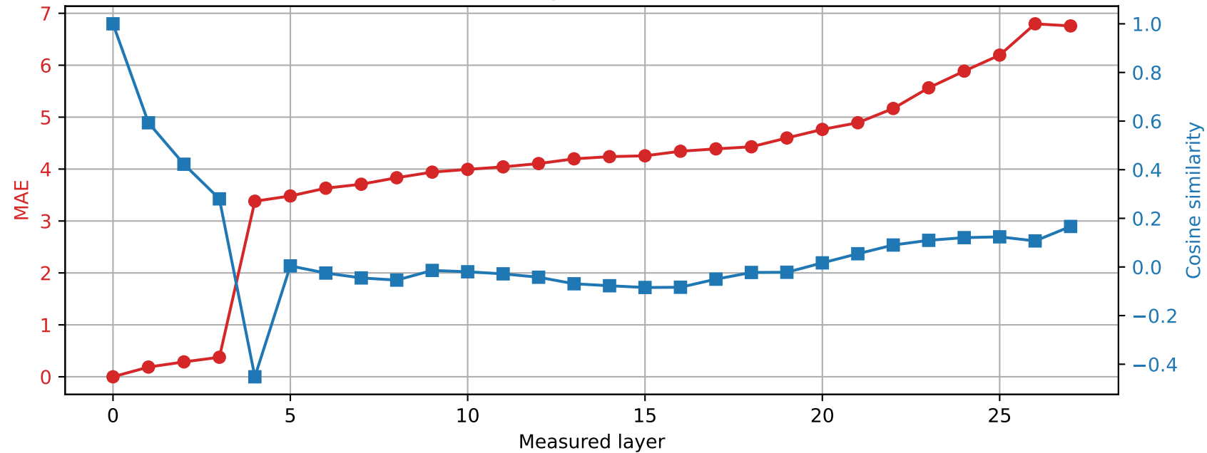
Qwen2.5-7B-Instruct | Prompt 4 Spared layer 22 | Hybrid vs unquantized
