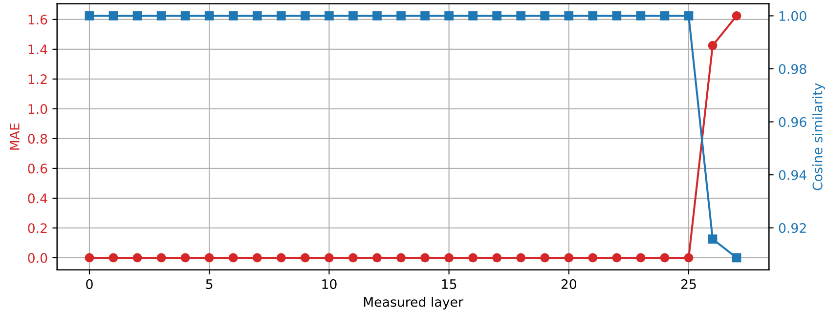
Qwen2.5-7B-Instruct | Prompt 4 Spared layer 25 | Hybrid vs quantized
