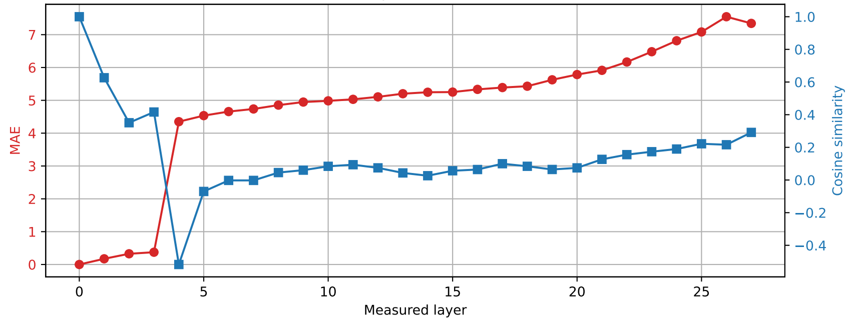
Qwen2.5-7B-Instruct | Prompt 0 Spared layer 2 | Hybrid vs unquantized
