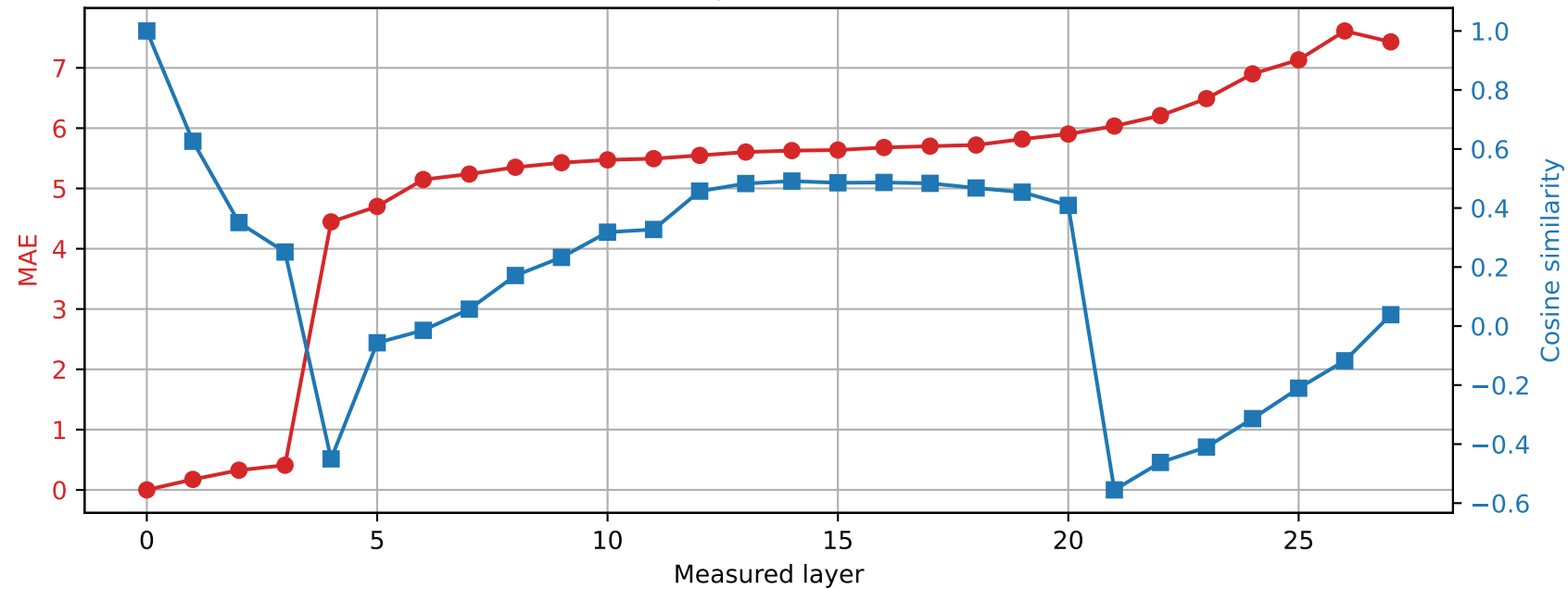
Qwen2.5-7B-Instruct | Prompt 0 Spared layer 23 | Hybrid vs unquantized
