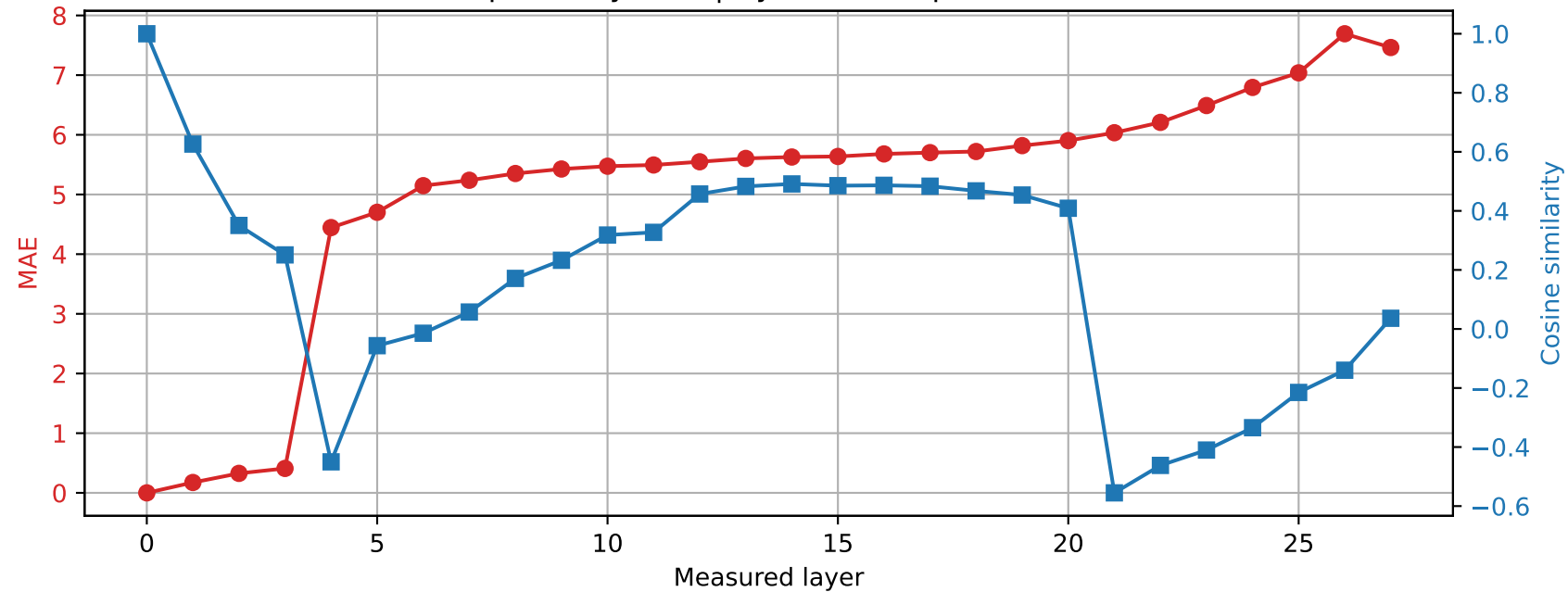
Qwen2.5-7B-Instruct | Prompt 0 Spared layer 25 | Hybrid vs unquantized
