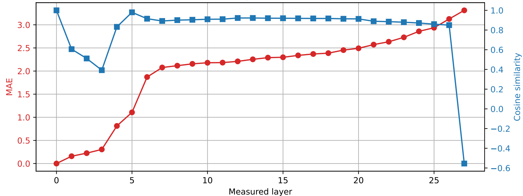
Qwen2.5-7B-Instruct | Prompt 1 Spared layer 0 | Hybrid vs quantized
