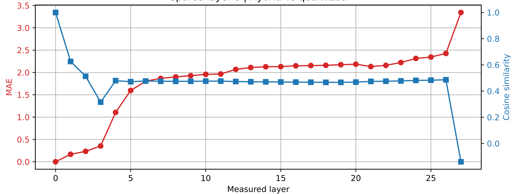
Qwen2.5-7B-Instruct | Prompt 2 Spared layer 0 | Hybrid vs quantized
