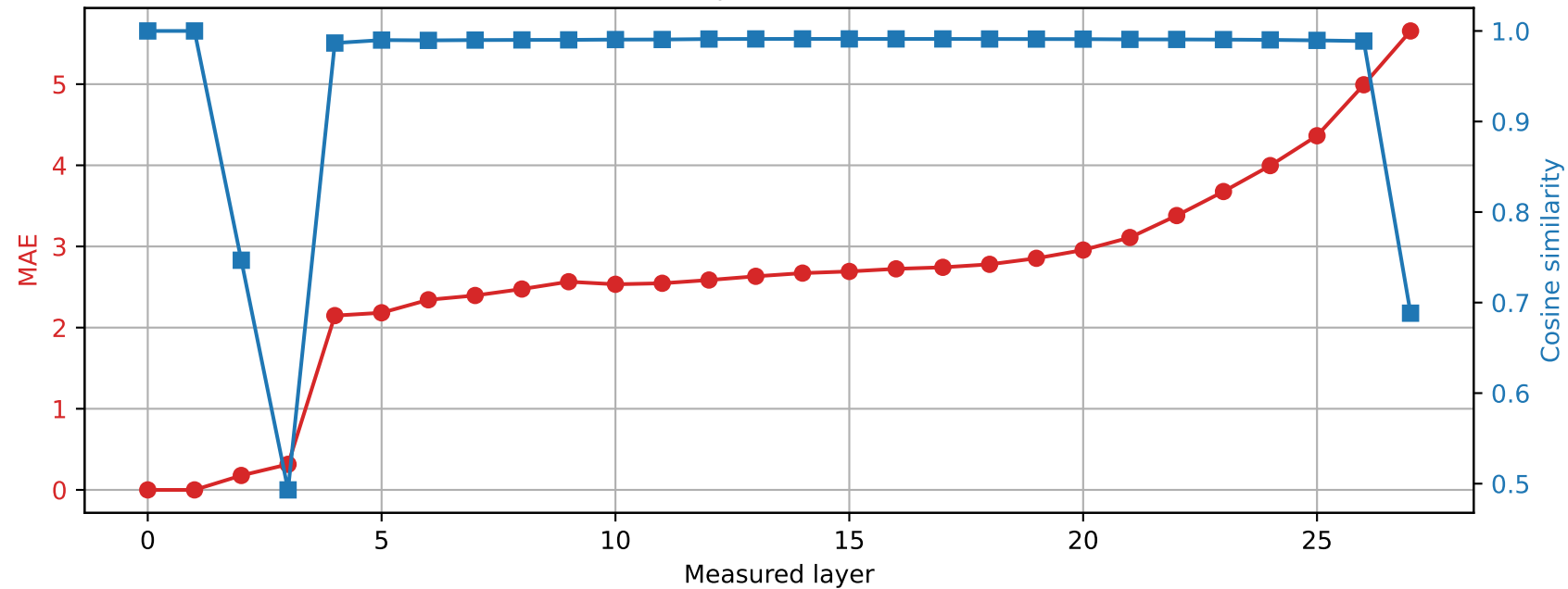
Qwen2.5-7B-Instruct | Prompt 2 Spared layer 0 | Hybrid vs unquantized
