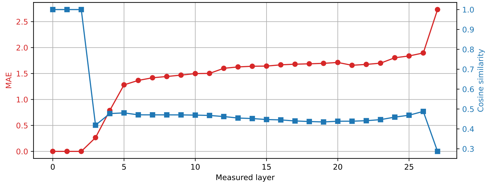
Qwen2.5-7B-Instruct | Prompt 2 Spared layer 2 | Hybrid vs quantized
