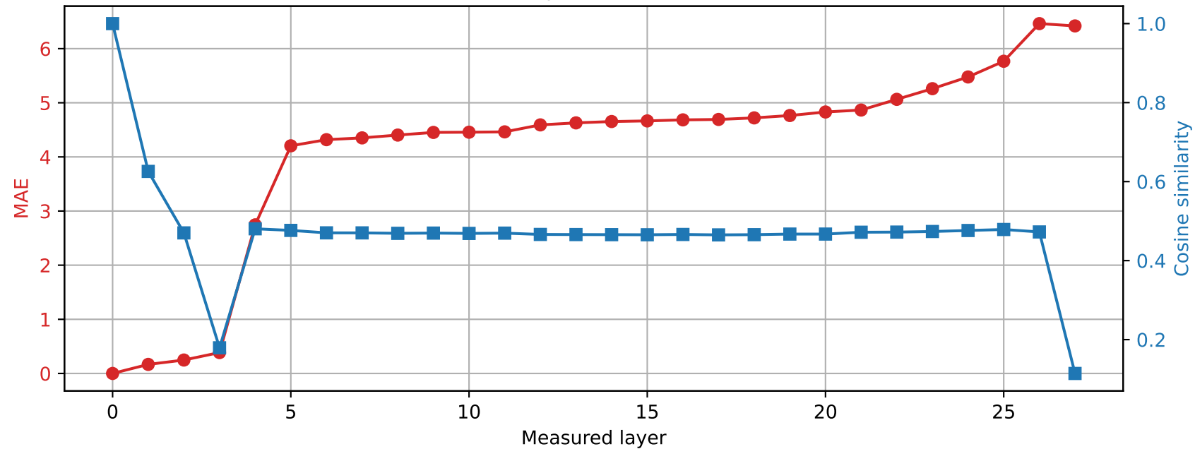
Qwen2.5-7B-Instruct | Prompt 2 Spared layer 4 | Hybrid vs unquantized
