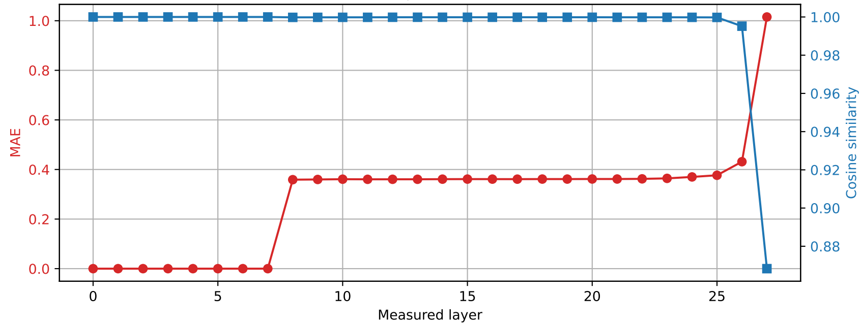
Qwen2.5-7B-Instruct | Prompt 2 Spared layer 7 | Hybrid vs quantized
