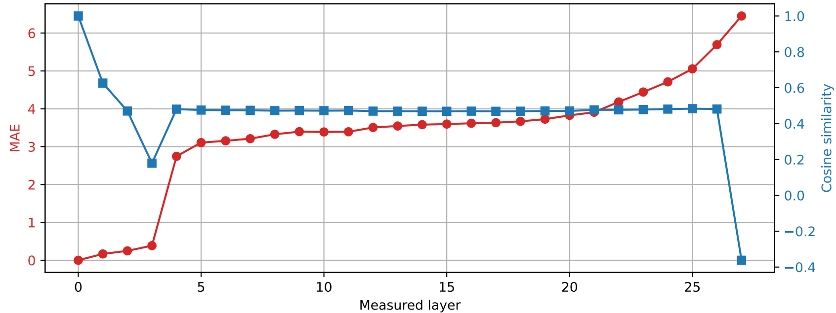
Qwen2.5-7B-Instruct | Prompt 2 Spared layer 7 | Hybrid vs unquantized
