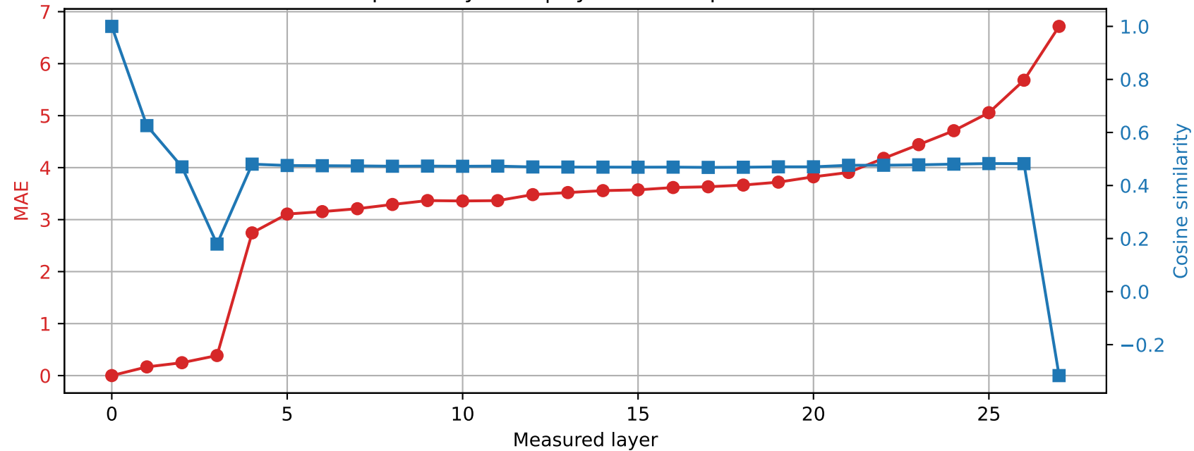
Qwen2.5-7B-Instruct | Prompt 2 Spared layer 15 | Hybrid vs unquantized
