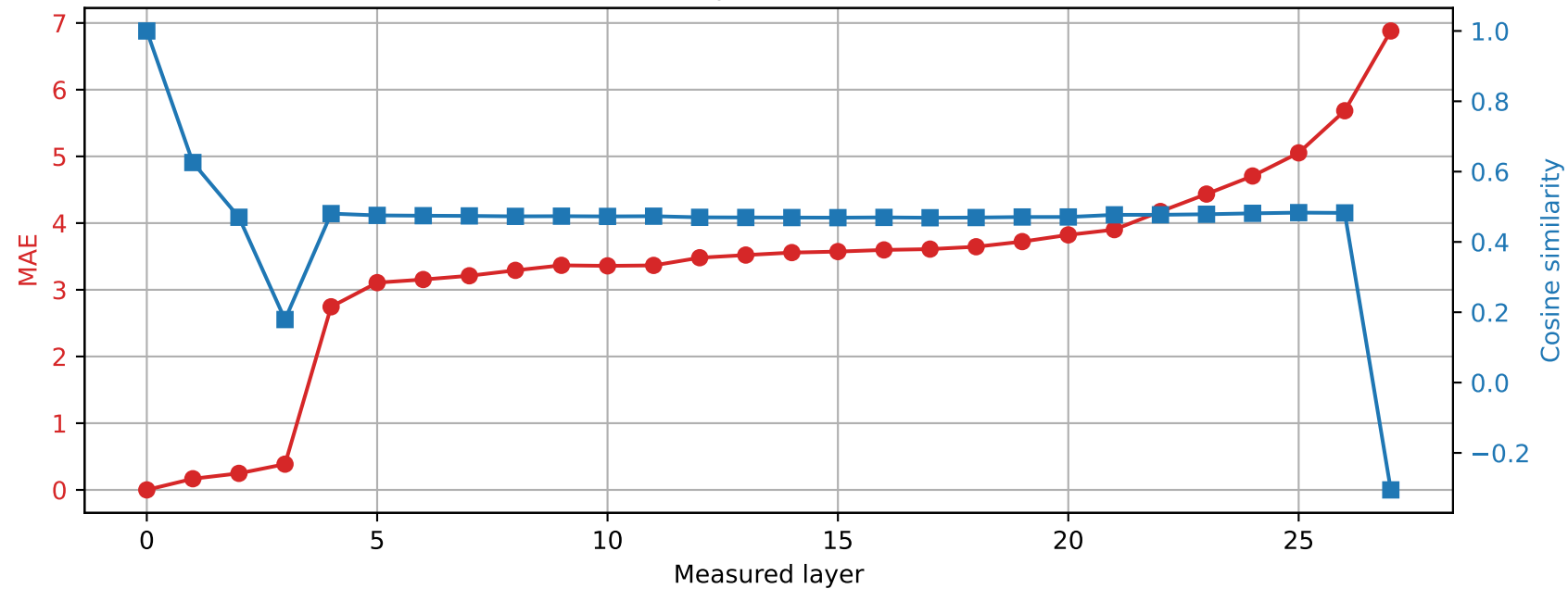
Qwen2.5-7B-Instruct | Prompt 2 Spared layer 18 | Hybrid vs unquantized
