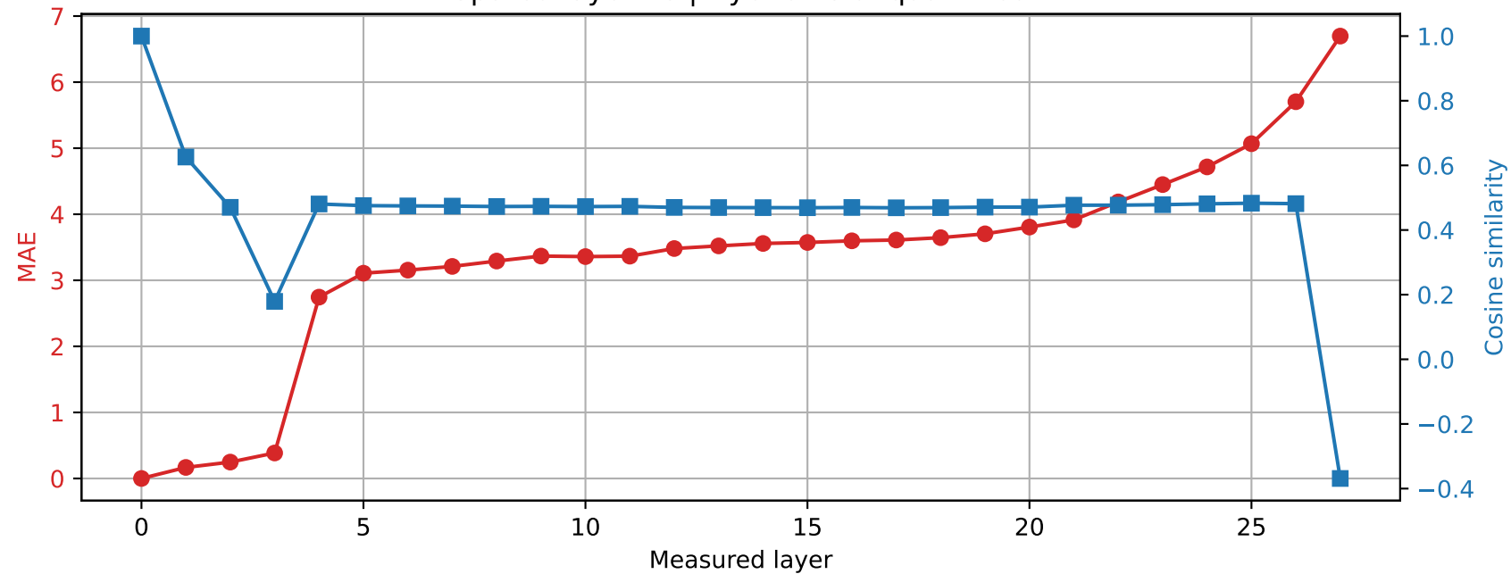
Qwen2.5-7B-Instruct | Prompt 2 Spared layer 20 | Hybrid vs unquantized
