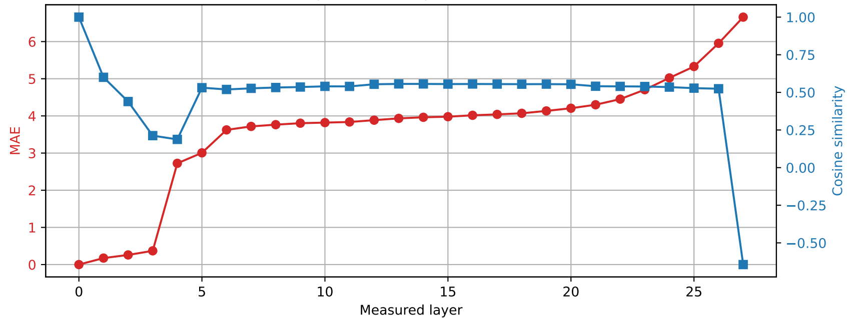
Qwen2.5-7B-Instruct | Prompt 3 Unquantized vs quantized int4
