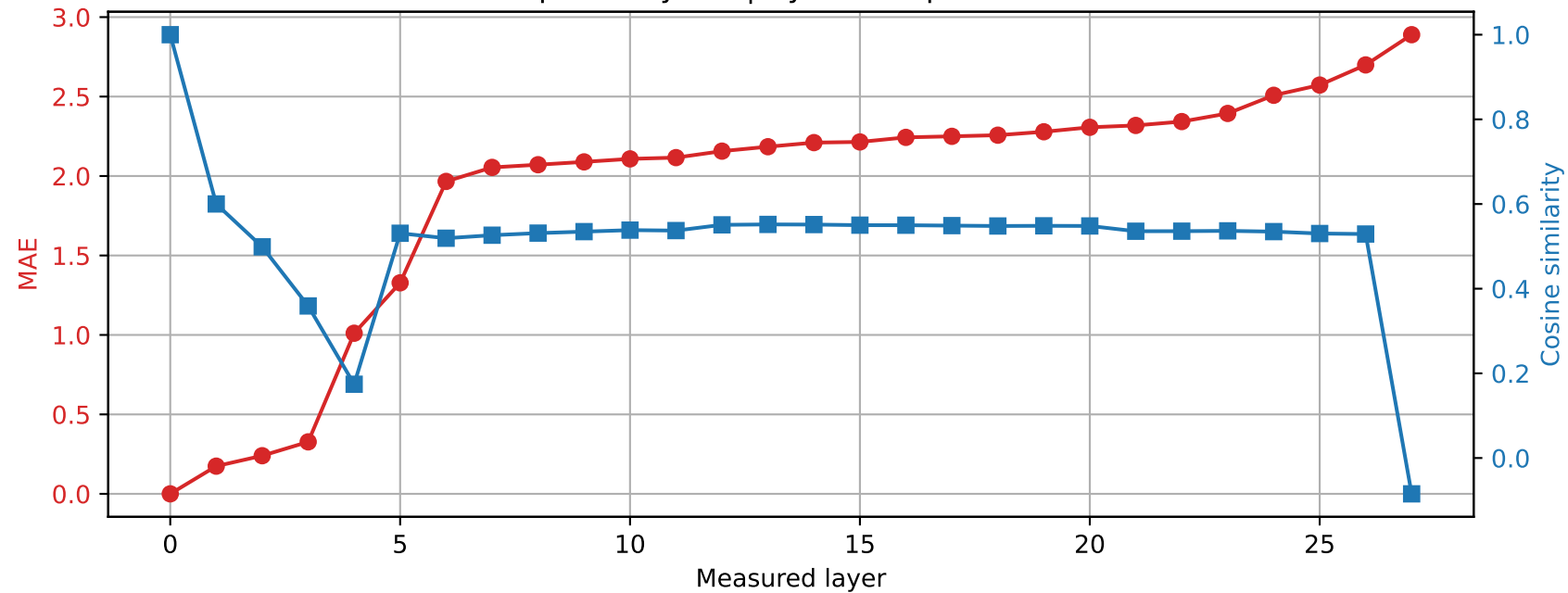
Qwen2.5-7B-Instruct | Prompt 3 Spared layer 0 | Hybrid vs quantized
