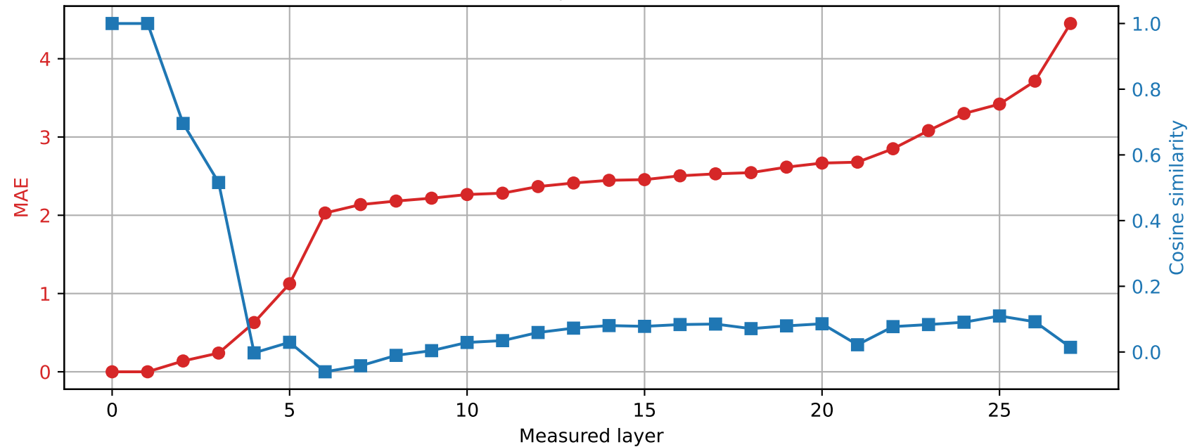
Qwen2.5-7B-Instruct | Prompt 3 Spared layer 1 | Hybrid vs quantized
