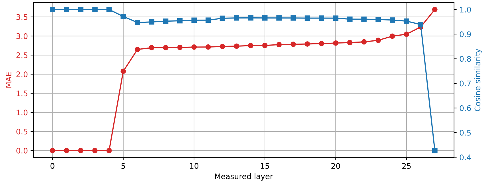
Qwen2.5-7B-Instruct | Prompt 3 Spared layer 4 | Hybrid vs quantized
