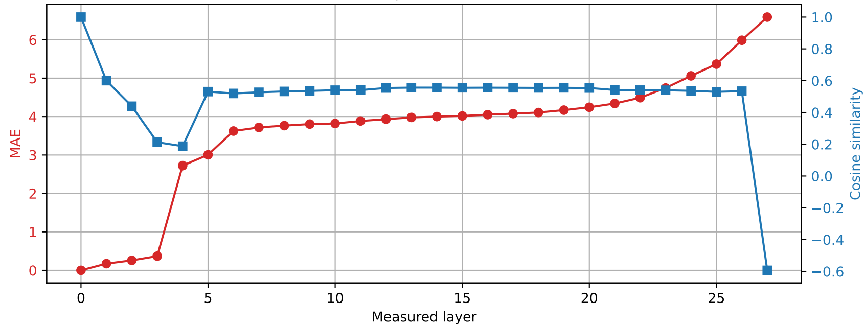
Qwen2.5-7B-Instruct | Prompt 3 Spared layer 10 | Hybrid vs unquantized
