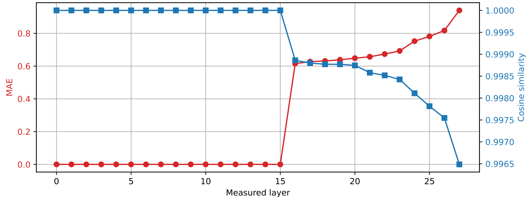
Qwen2.5-7B-Instruct | Prompt 3 Spared layer 15 | Hybrid vs quantized
