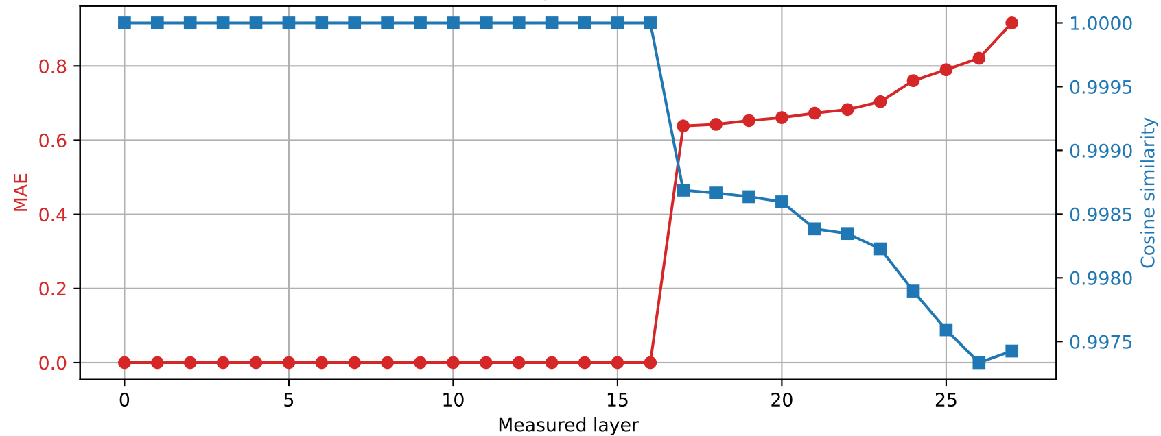
Qwen2.5-7B-Instruct | Prompt 3 Spared layer 16 | Hybrid vs quantized
