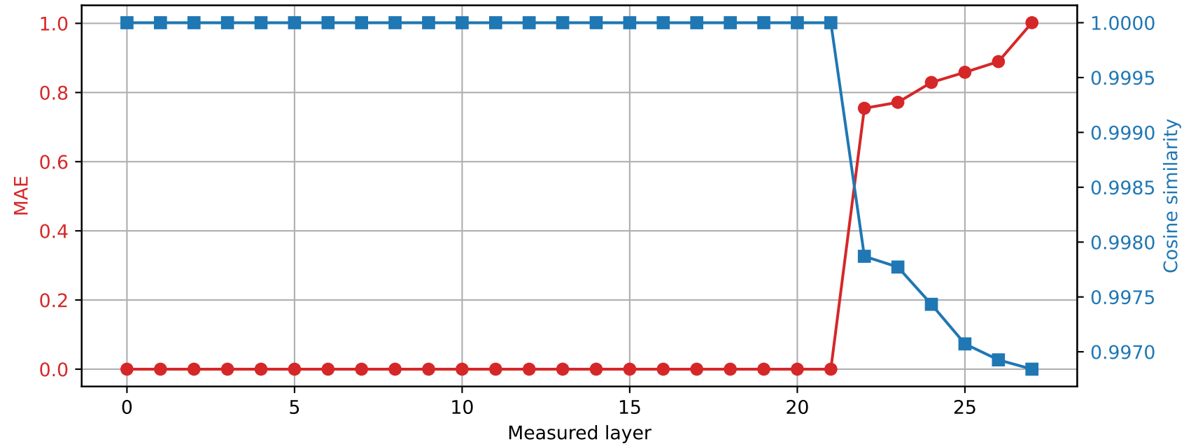
Qwen2.5-7B-Instruct | Prompt 3 Spared layer 21 | Hybrid vs quantized
